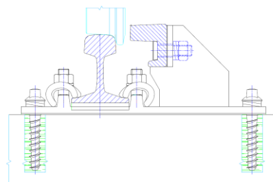
Section in area of guide-rail location
