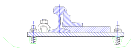
Section of the switch at the beginning of the tongue
