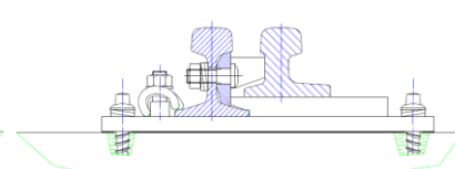
Section in area of tongue support
