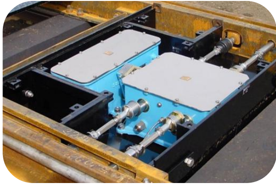
automatic point system VSP-1-K
