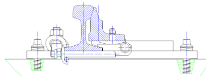
Section of the switch in area of roller idler
