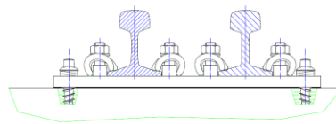
Section in area of switch end
